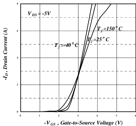
Fig 11. Transfer Characteristics
