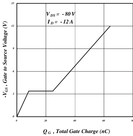
Fig 7. Gate Charge Characteristics
