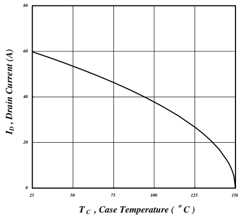
Fig 12. Maximum Continuous Drain Current v.s. Case Temperature
