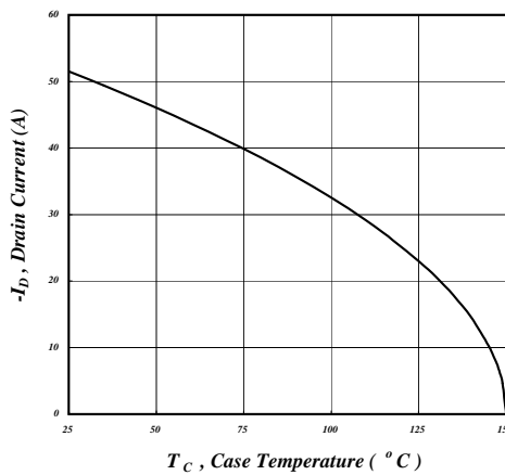
Fig 11. Maximum Continuous Drain Current v.s. Case Temperature
