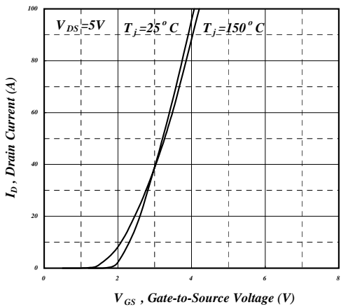
Fig 11. Transfer Characteristics
