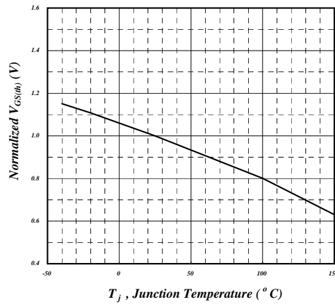
Fig 6. Gate Thres. Junction Temperature
