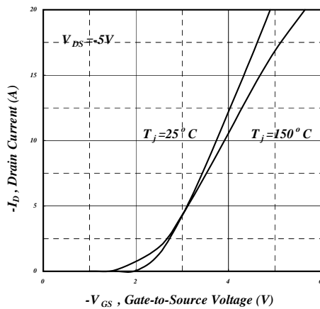
Fig 11. Transfer Characteristics
