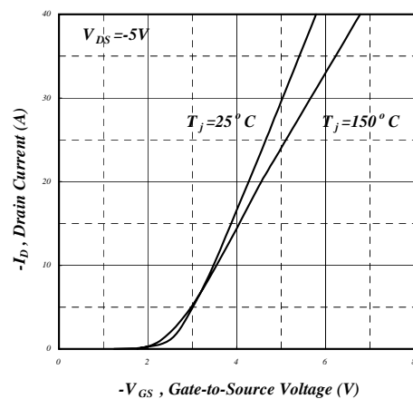
Fig 11. Transfer Characteristics
