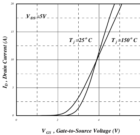
Fig 11. Transfer Characteristics
