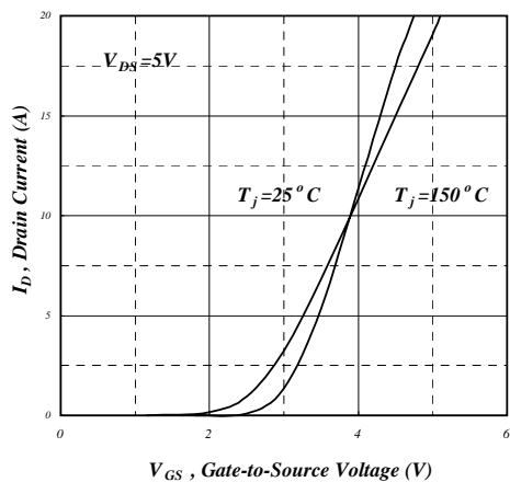
Fig 11. Transfer Characteristics
