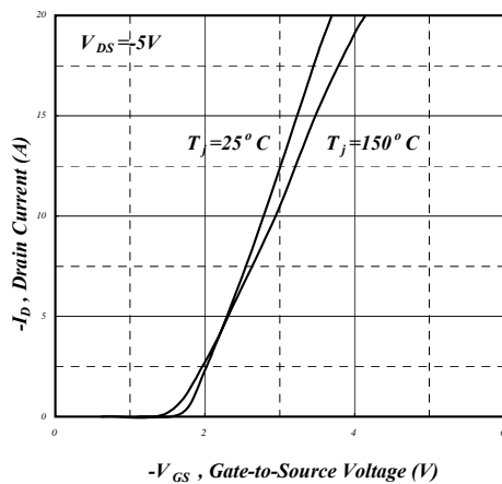
Fig 11. Transfer Characteristics
