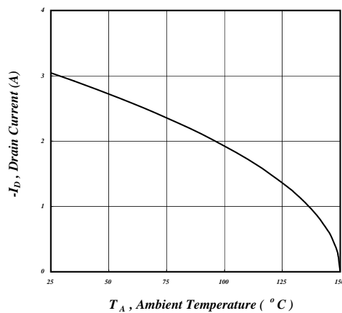
Fig 11. Maximum Continuous Drain Current v.s. Ambient Temperature
