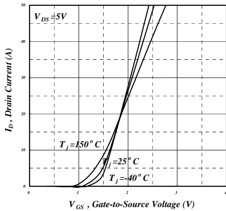
Fig 11. Transfer Characteristics
