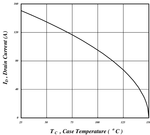
Fig 11. Maximum Continuous Drain Current v.s. Case Temperature
