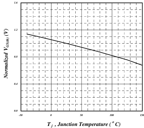
Fig 6. Gate Thresh. Voltage v.s. Junction Temperature
