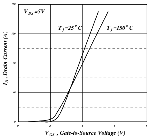
Fig 11. Transfer Characteristics
