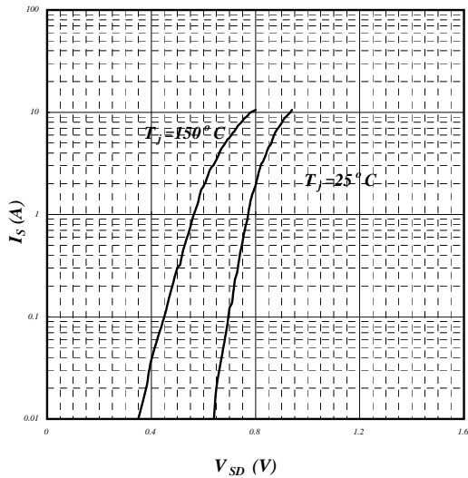
Fig 11. Forward Characteristic of Reverse Diode
