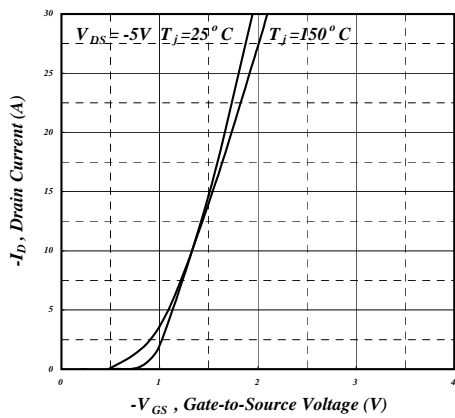
Fig 11. Transfer Characteristics
