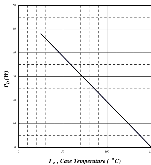
Fig 6. Typical Power Dissipation
