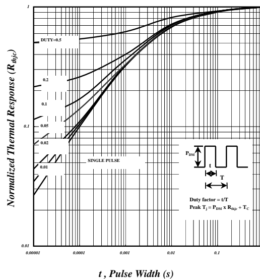
Fig 8. Effective Transient Thermal Impedance
