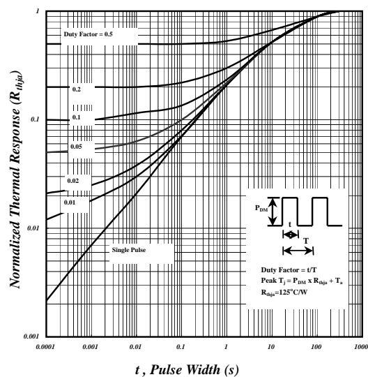
Fig 8. Effective Transient Thermal Impedance
