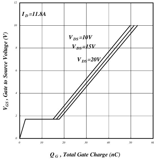
Fig 9. Gate Charge Characteristics
