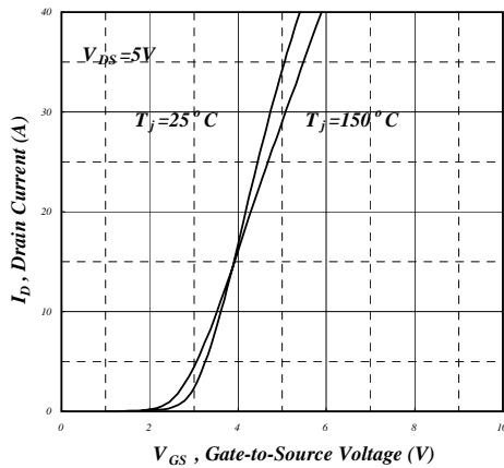
Fig 11. Transfer Characteristics
