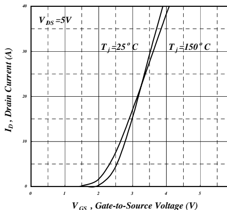
Fig 6. Transfer Characteristics
