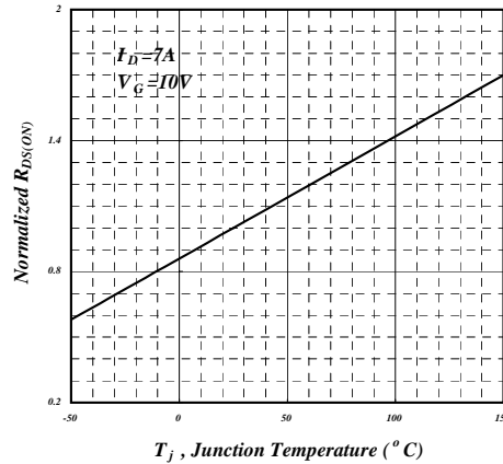
Fig 4. Normalized On-Resistance
