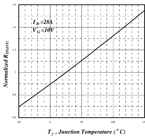
Fig 4. Normalized On-Resistance
