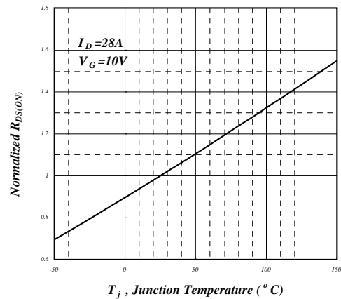
Fig 4. Normalized On-Resistance
