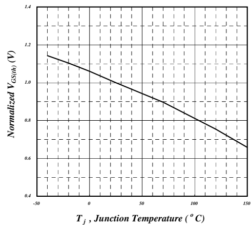
Fig 6. Gate Thres. Voltage v.s. Junction Temperature
