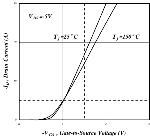
Fig 11. Transfer Characteristics
