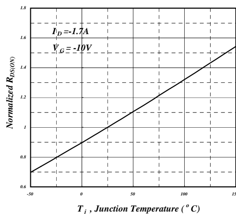
Fig 4. Normalized On-Resistance
