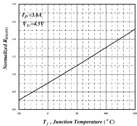
Fig 4. Normalized On-Resistance
