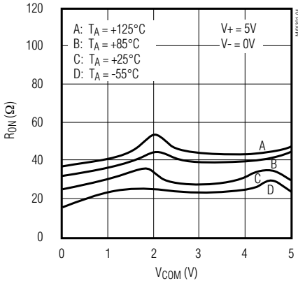
RON vs. VCOM AND TEMPERATURE (SINGLE SUPPLY)
