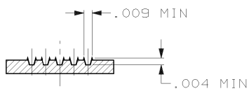
SECTION C-C SCALE 10:1
