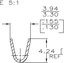
SECTION B-B SCALE 5:1
