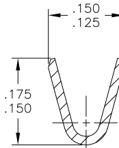
SECTION X-X SCALE 8:1
