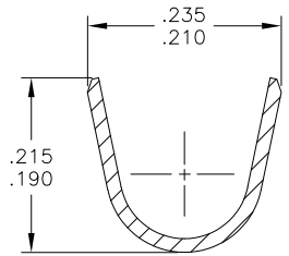
SECTION Y-Y SCALE 8:1
