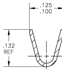
SECTION B-B SCALE 10:1
