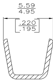
SECTION A-A SCALE 8:1
