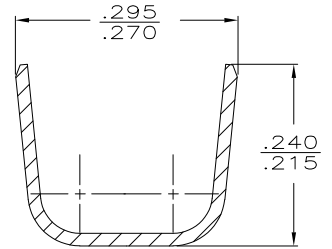
SECTION C-C SCALE 5:1
