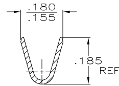
SECTION B-B SCALE 5:1
