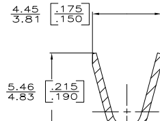
SECTION B-B SCALE 8:1
