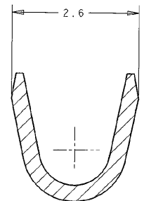
SECTION C-C SCALE 20:1
