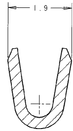
SECTION B-B SCALE 20:1
