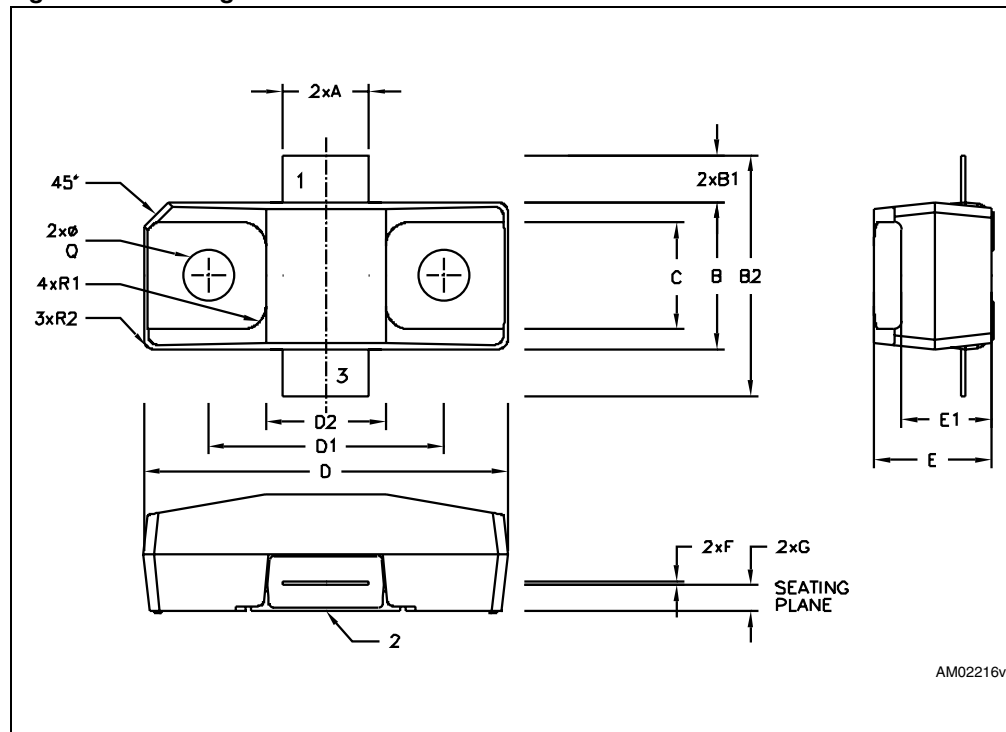
Figure 12. Package dimensions
