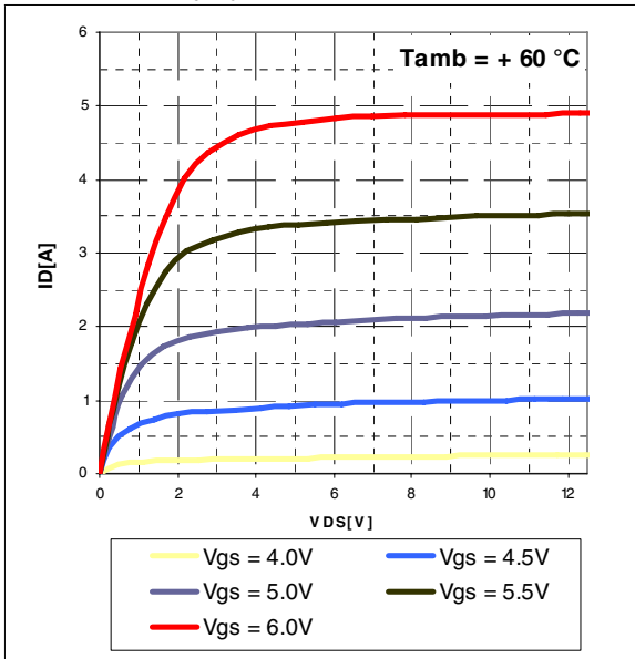
Figure 6. DC output characteristics ( T_{amb} = 60\text{ }^{\circ}\text{C} )
