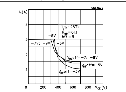
Figure 5. Reverse biased safe operating areas
