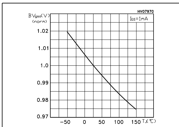
Figure 17. Normalized BV gs0 vs temperature
