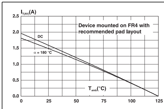
Figure 3. Average DC on-state current versus ambient temperature
