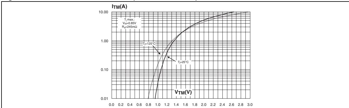
Figure 15. On-state characteristics (maximum values)
