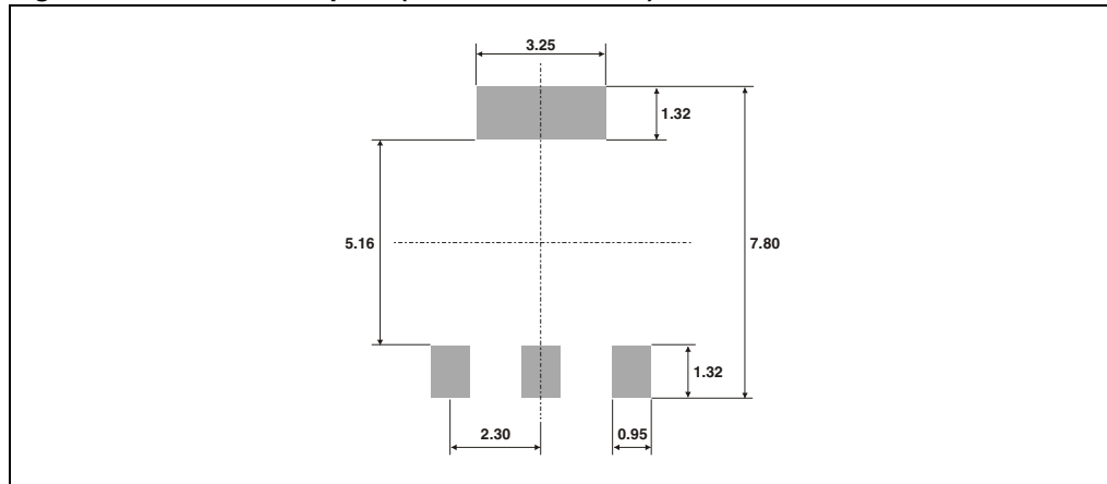
Figure 17. SOT-223 footprint (dimensions in mm)
