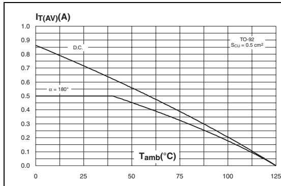
Figure 3. Average and D.C. on-state current versus ambient temperature (epoxy printed circuit board FR4, copper thickness = 35 μm, S CU = 0.5 cm 2 ) (TO-92)
