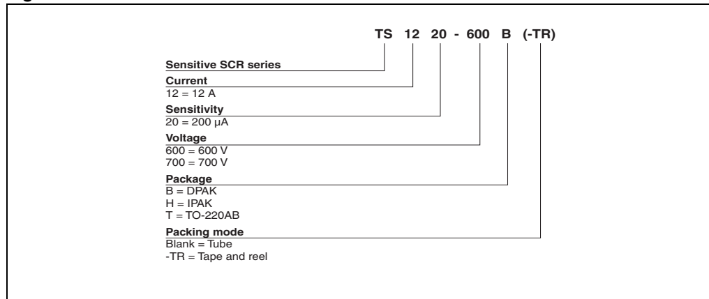
Figure 16. TS1220 series
