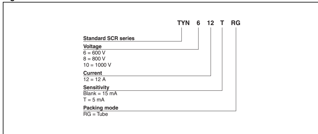
Figure 17. TYNx12 series
