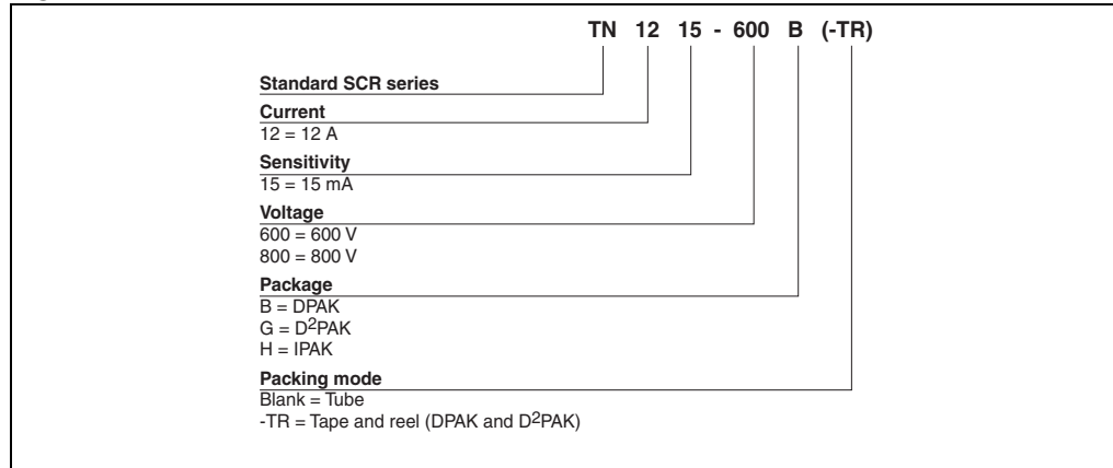
Figure 15. TN1215 series
