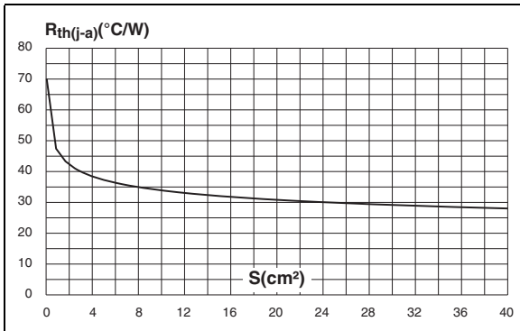
Figure 9. Thermal resistance junction to ambient versus copper surface under tab (epoxy printed circuit board FR4, copper thickness: 35 \mu\text{m} ) ( \text{D}^2\text{PAK} )
