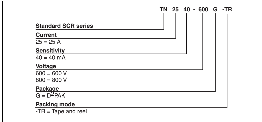
Figure 12. TXN625RG ordering information scheme
