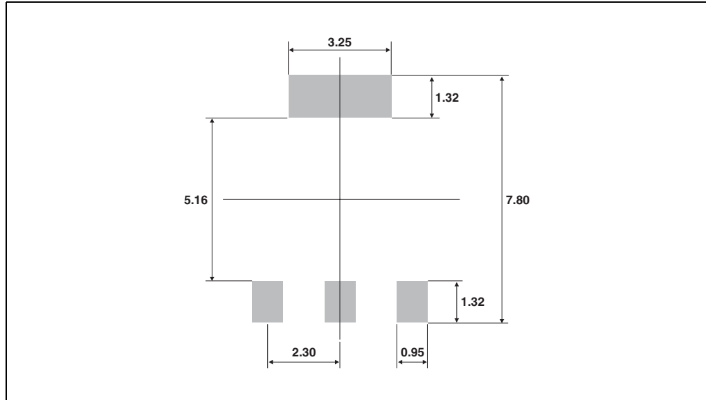
Figure 22. SOT-223 footprint
