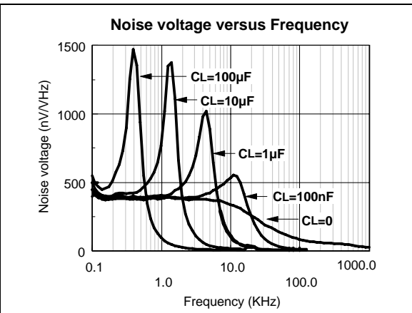
Figure 6. Noise voltage versus frequency
