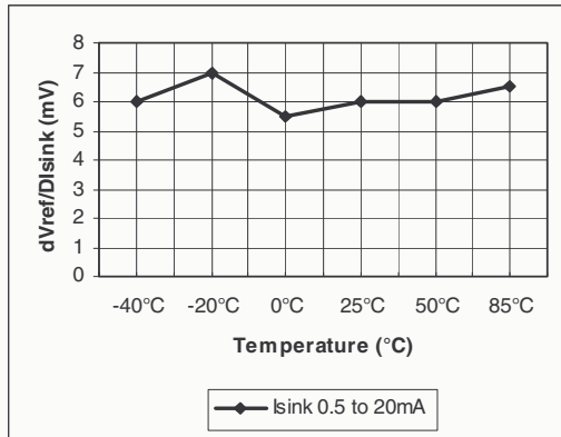
Figure 8. dV_{ref}/dI_{sink} vs. temp. V_{cc}=1.8V
