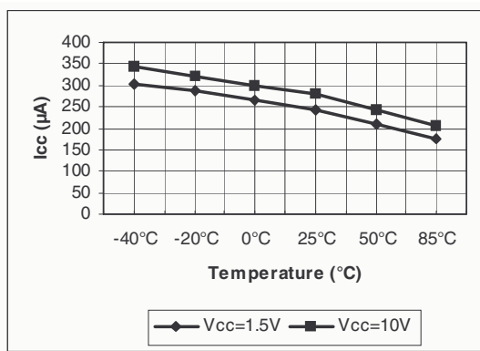
Figure 6. Icc vs. temp. Isink=2mA
