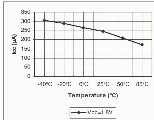
Figure 5. Icc vs. temp. Isink=2mA
