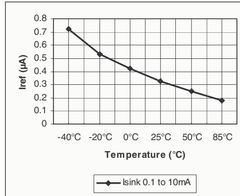
Figure 9. I_{ref} vs. temp. V_{cc}=1.8V
