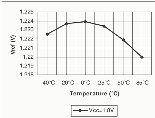
Figure 2. Vref vs. temp. Isink=2mA
