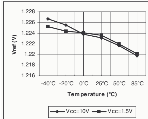
Figure 3. Vref vs. temp. Isink=2mA
