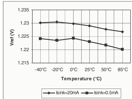
Figure 7. Vref vs. temp. Vcc=1.8V
