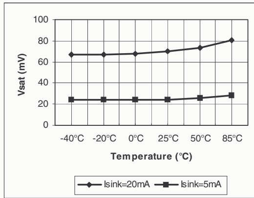
Figure 10. V_{sat} vs. temp. V_{cc}=1.8V
