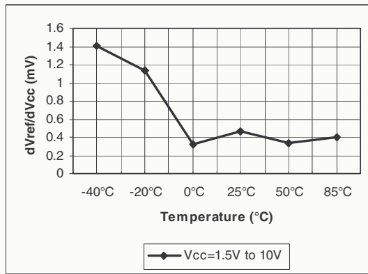
Figure 4. dVref/dVcc vs. temp. Isink=2mA
