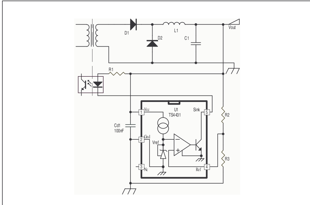
Figure 1. SMPS power supply: secondary side
