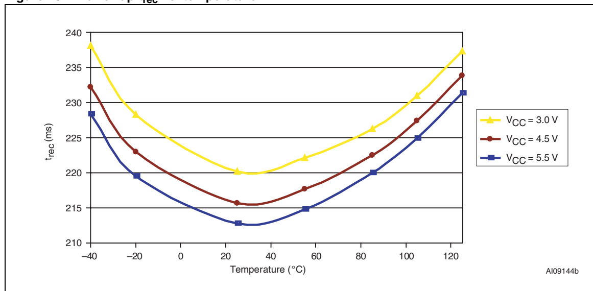
Figure 15. Power-up t_{\text{rec}} vs. temperature
