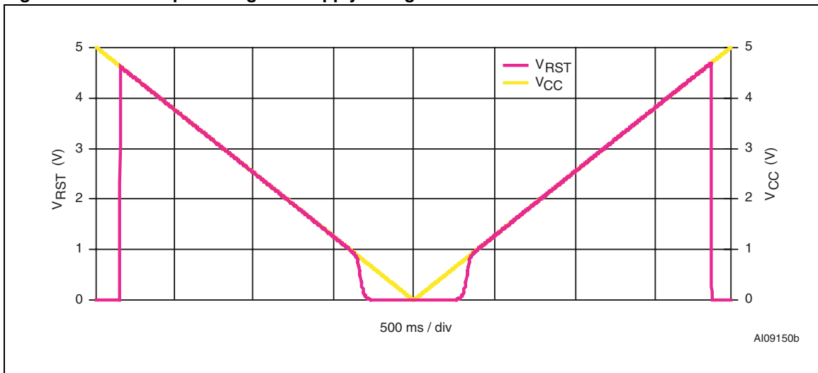
Figure 21. RST output voltage vs. supply voltage
