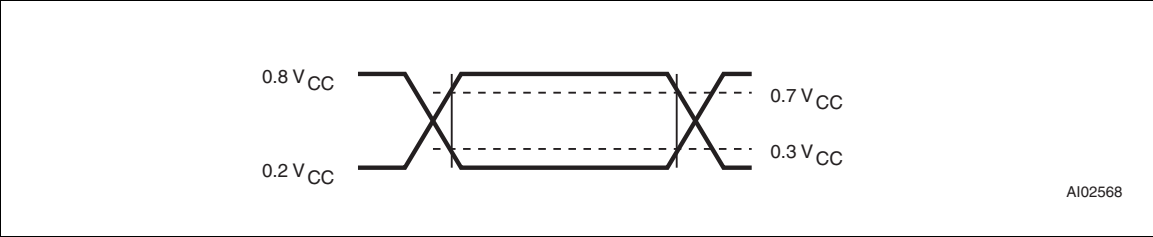
Figure 27. AC testing input/output waveforms
