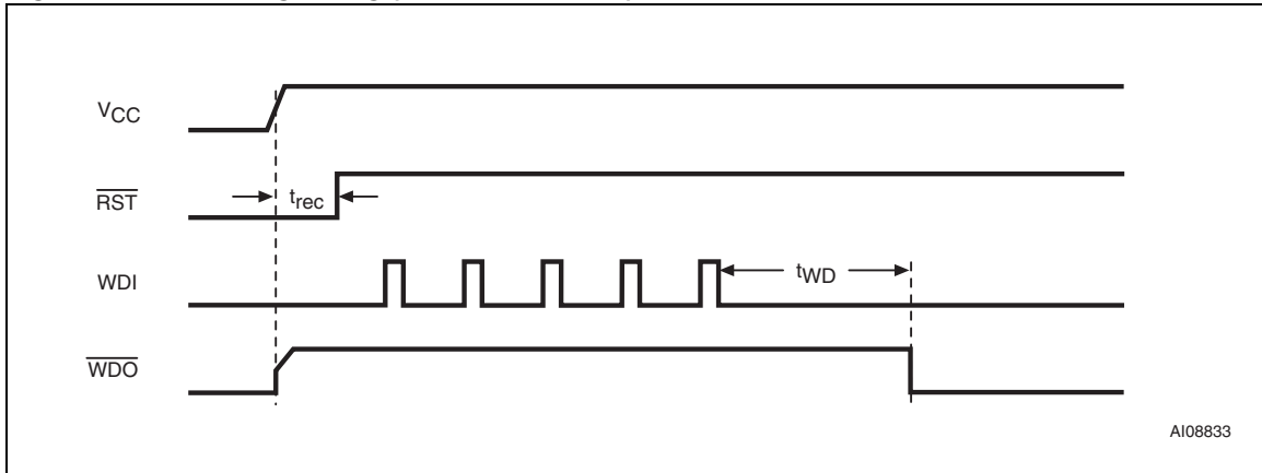
Figure 30. Watchdog timing (STM705/706/813L)
