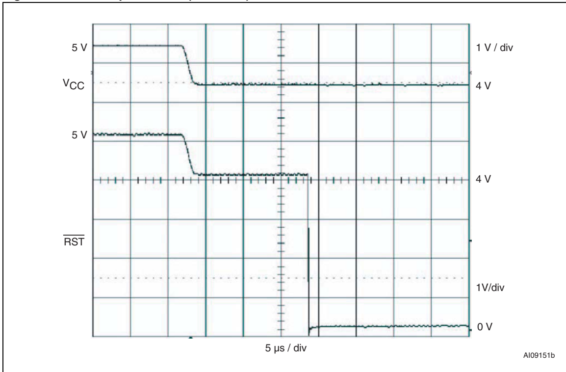
Figure 22. \overline{\text{RST}} response time (assertion)
