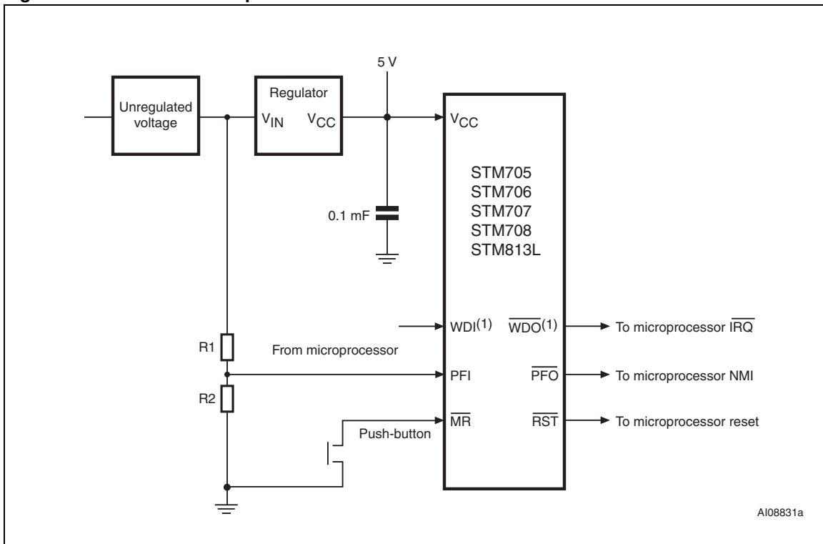
Figure 9. Hardware hookup
